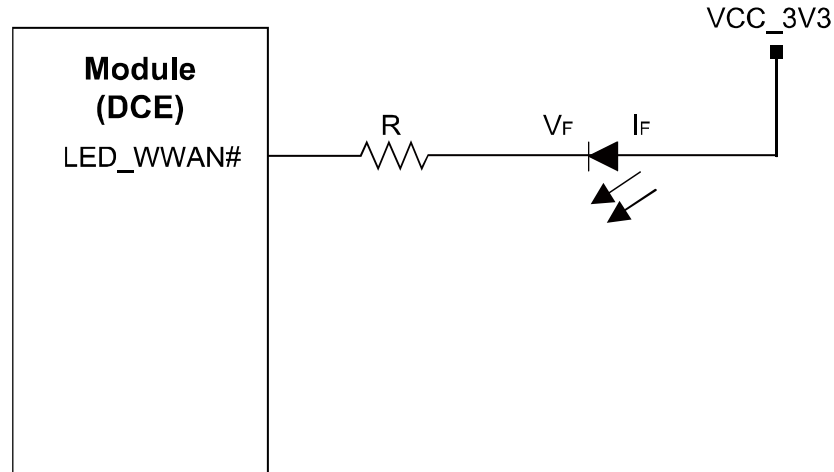
Figure 3-7 Driving circuit
