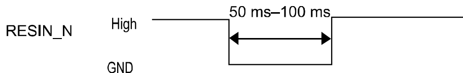
Figure 3-6 Reset pulse time sequence
