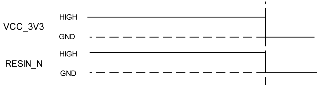
Figure 3-3 Power off time sequence
