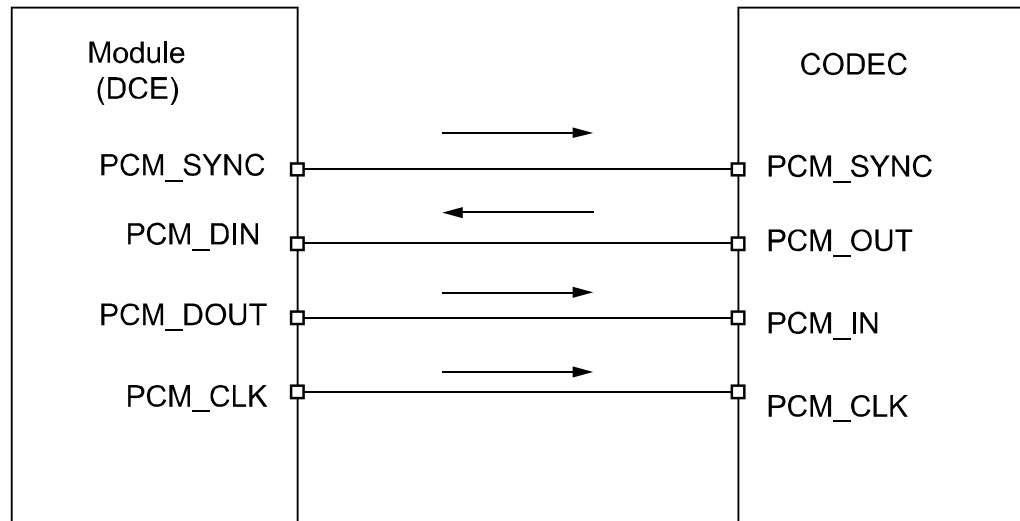
Figure 3-10 Circuit diagram of the interface of the PCM (ME209u-526 Mini PCIe module is used as PCM master)
