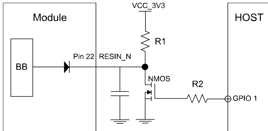
Figure 3-5 Connections of the RESIN_N pin
