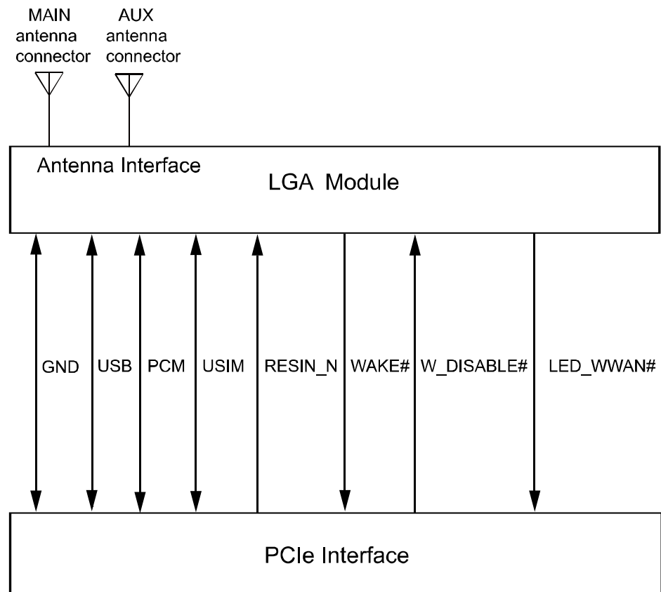
Figure 2-1 Circuit block diagram of the ME209u-526 Mini PCIe module
