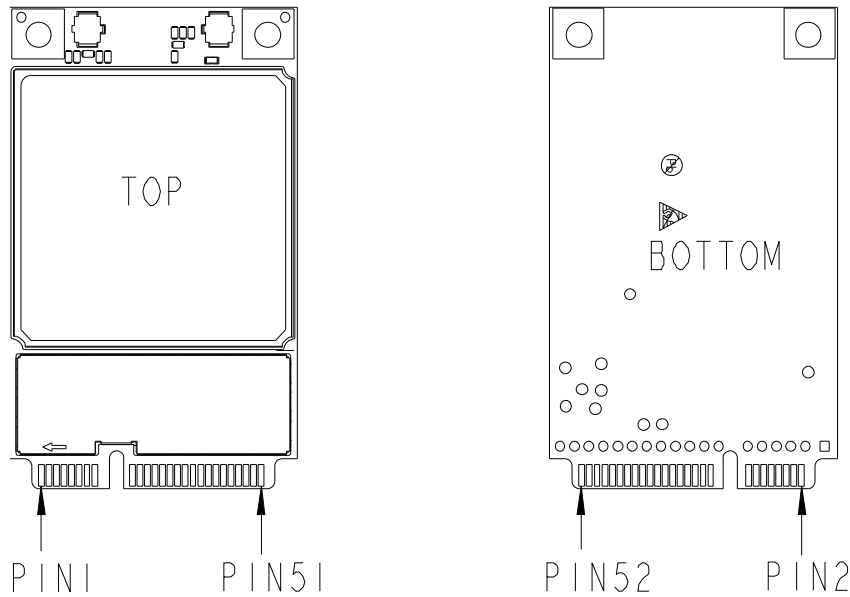
Figure 3-1 Appearance of Mini PCIe interface
