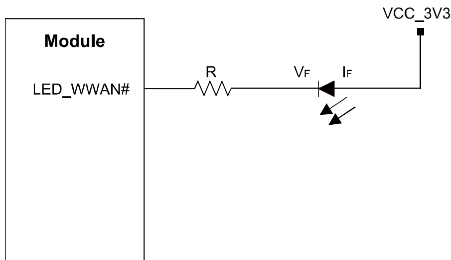
Figure 3-7 Driving circuit
