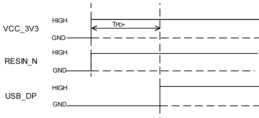
Figure 3-2 Power on time sequence
