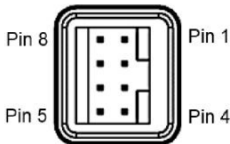
MFC2030 pin configuration.
